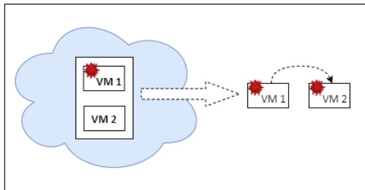
FIGURE 7 Level 1: Collateral damages on sibling VM's inside the same host 19
