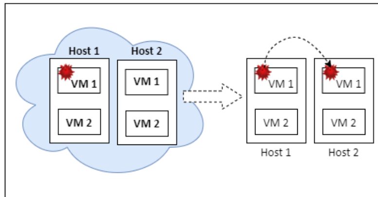
FIGURE 8 Level 2: Collateral damages at the sibling host level and on its VMs 19
